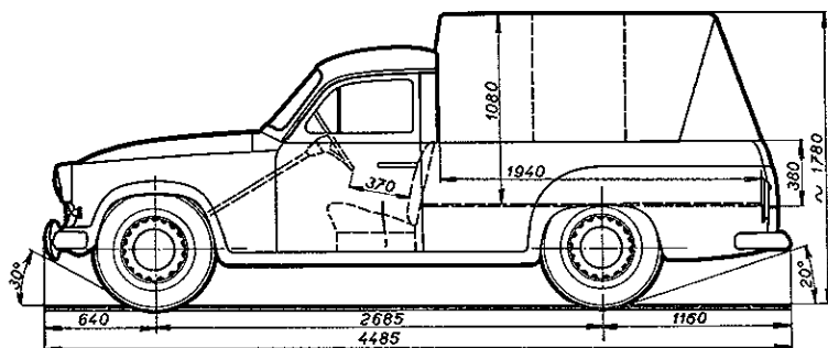
Automobil ŠKODA 1202 — PICK-UP
